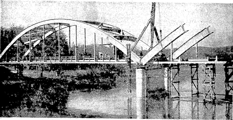
The tempo of construction on the Grand Detour bridge has increased with improved weather—the winter months having practically halted operations. The scene here shows the beginning of the second span with two of the girders being placed in position.
